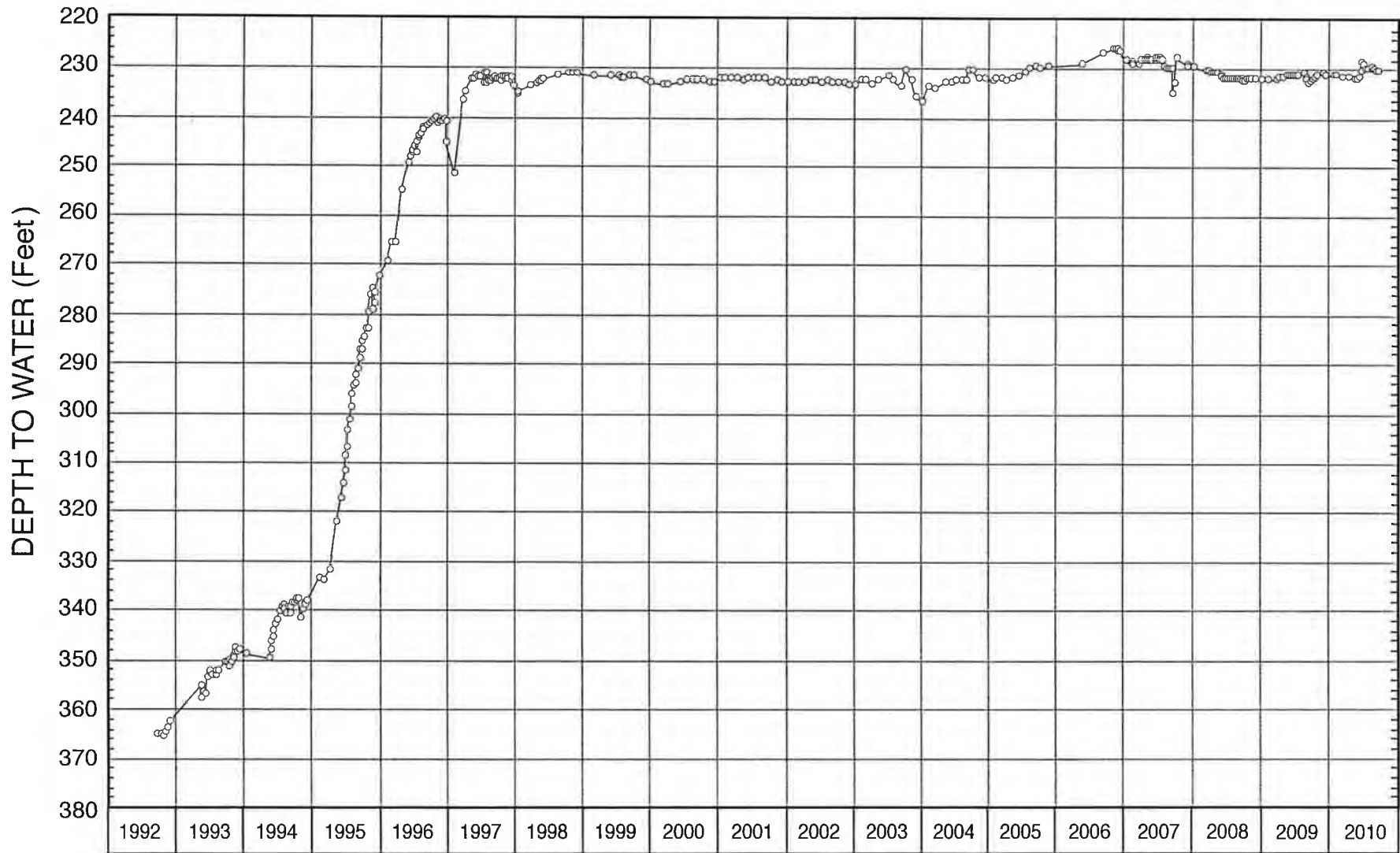
FIGURE 10 - WATER-LEVEL HYDROGRAPH FOR WELL NO. 21
