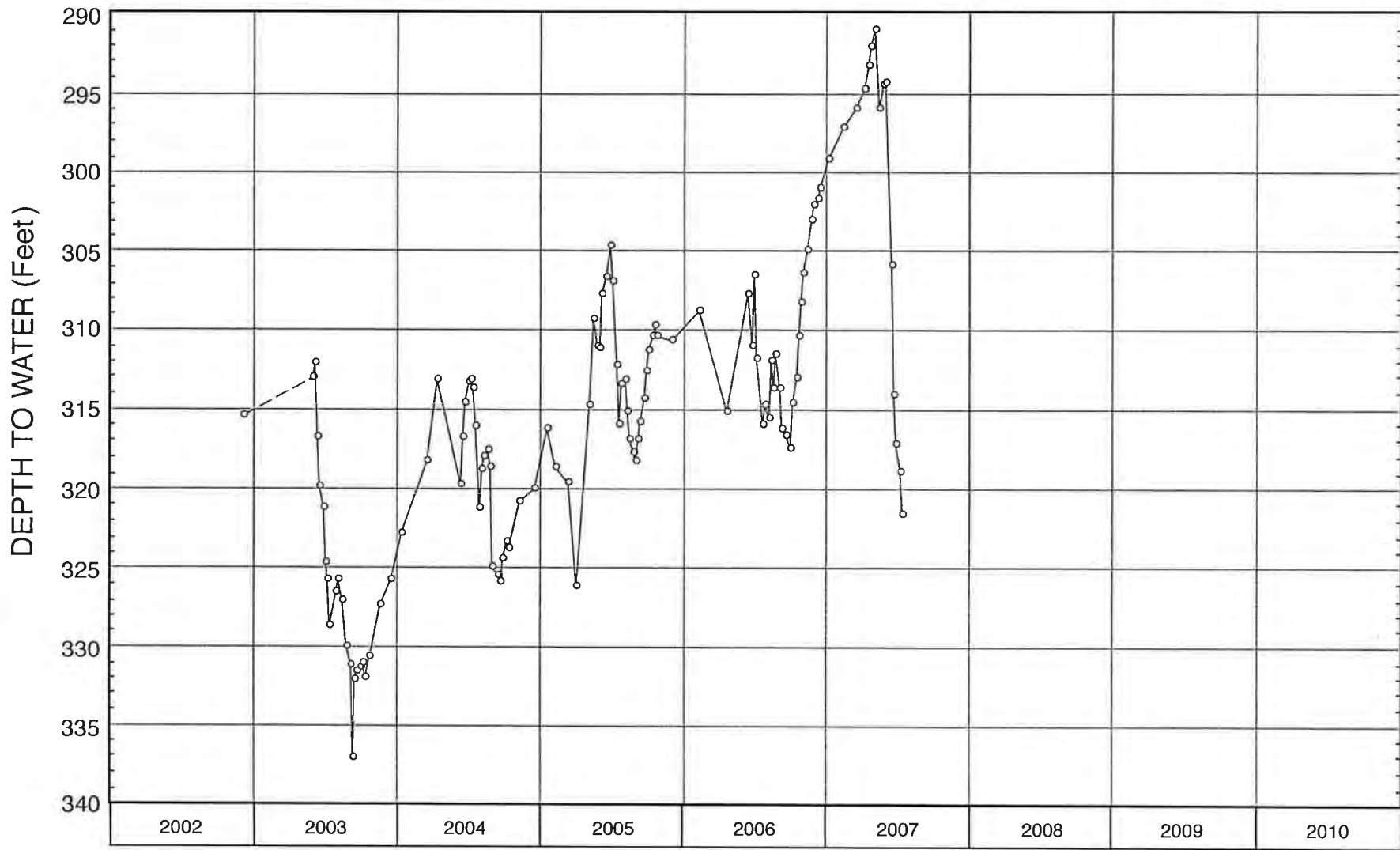
WATER-LEVEL HYDROGRAPH FOR WELL NO. 25
