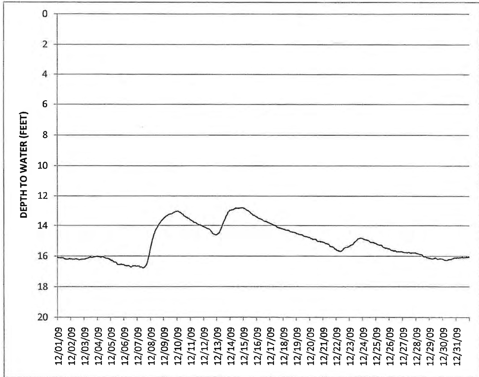
WATER LEVEL HYDROGRAPH FOR MW-23M
