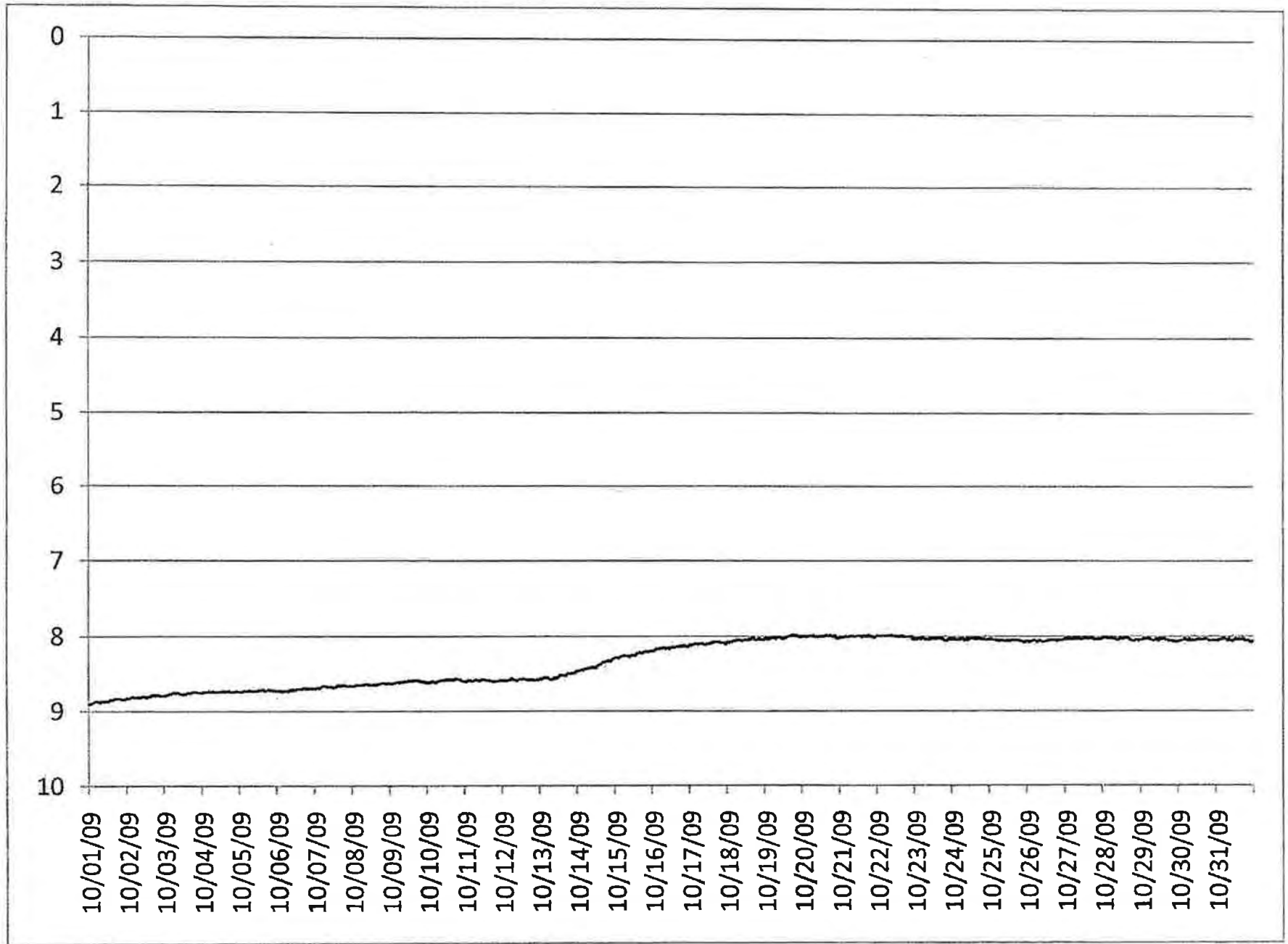
WATER LEVEL HYDROGRAPH FOR MW-5M
