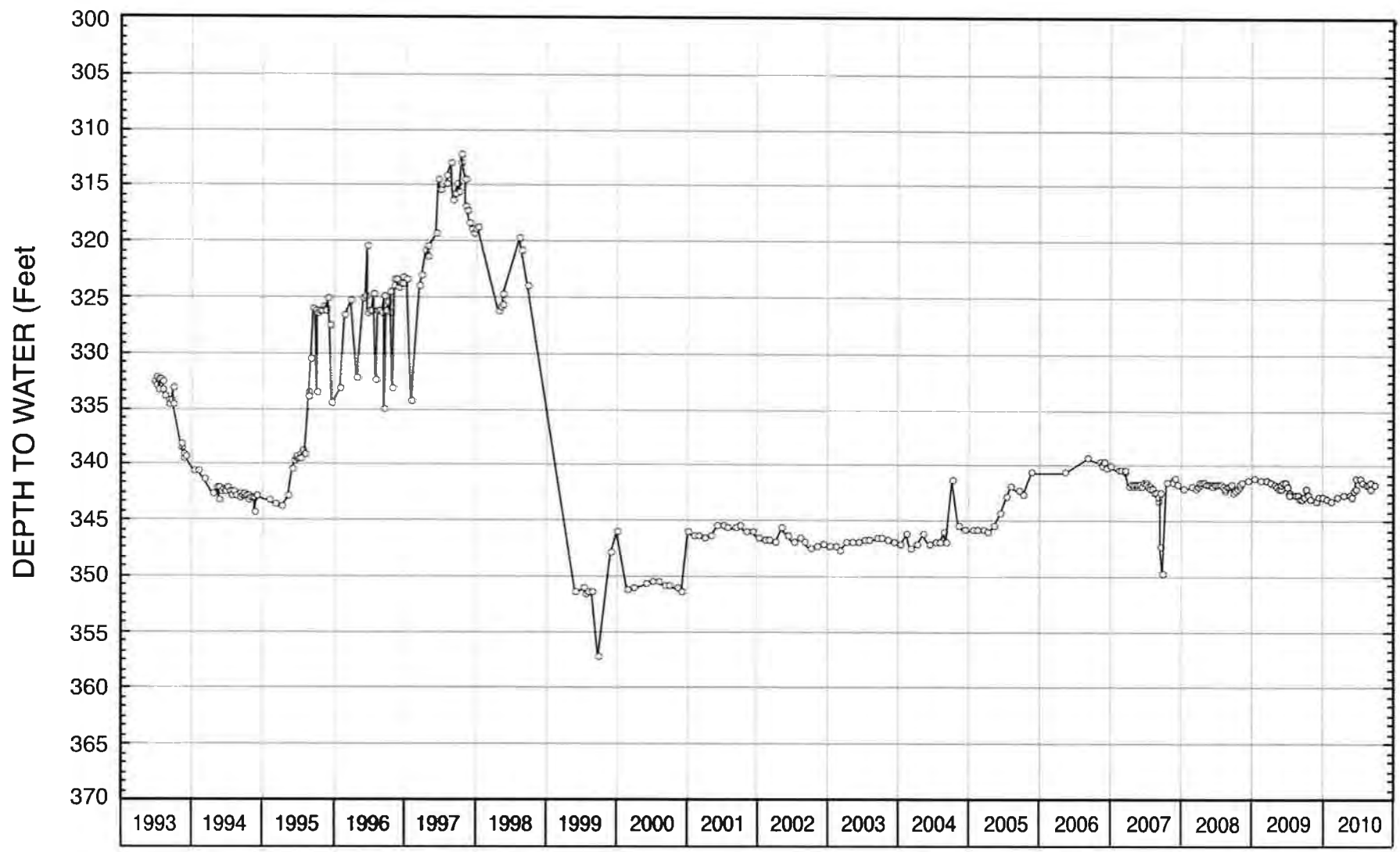
FIGURE 9 - WATER-LEVEL HYDROGRAPH FOR WELL NO. 19
