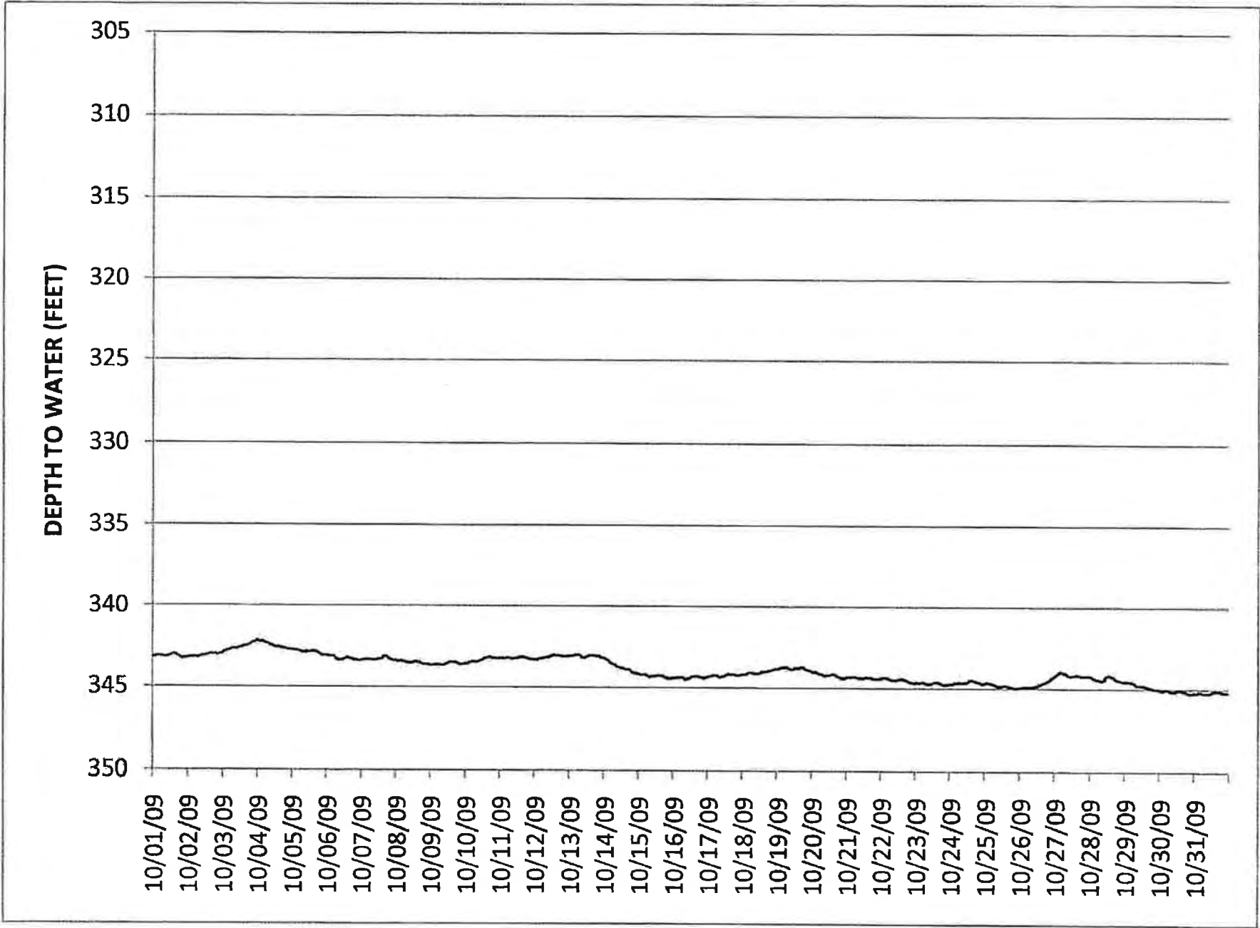
WATER LEVEL HYDROGRAPH FOR MW-14M
