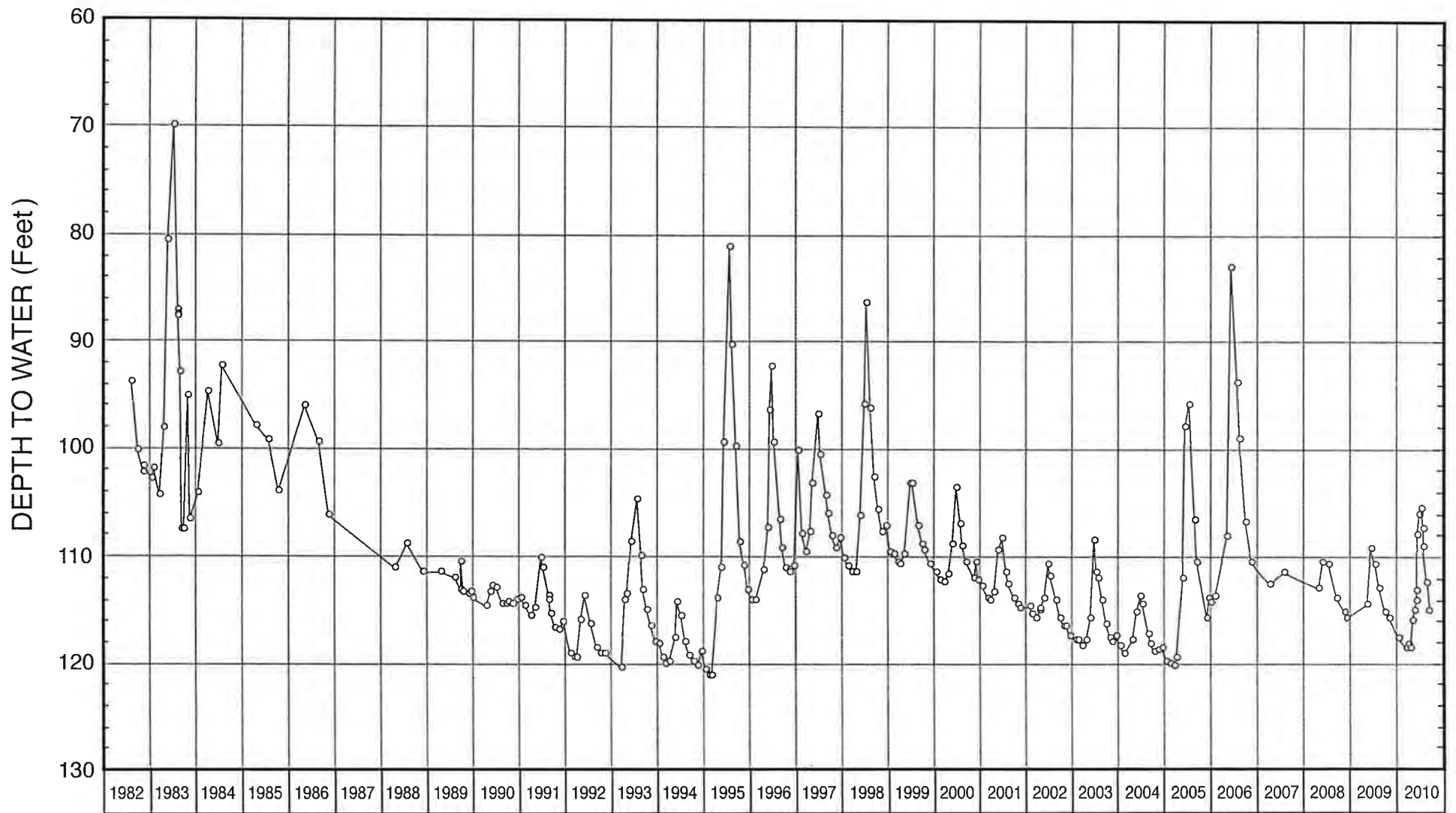
FIGURE 12 - WATER-LEVEL HYDROGRAPH FOR SC-1
