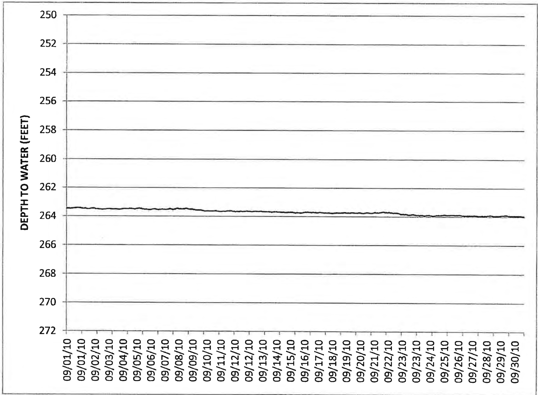
WATER LEVEL HYDROGRAPH FOR MW-26M
