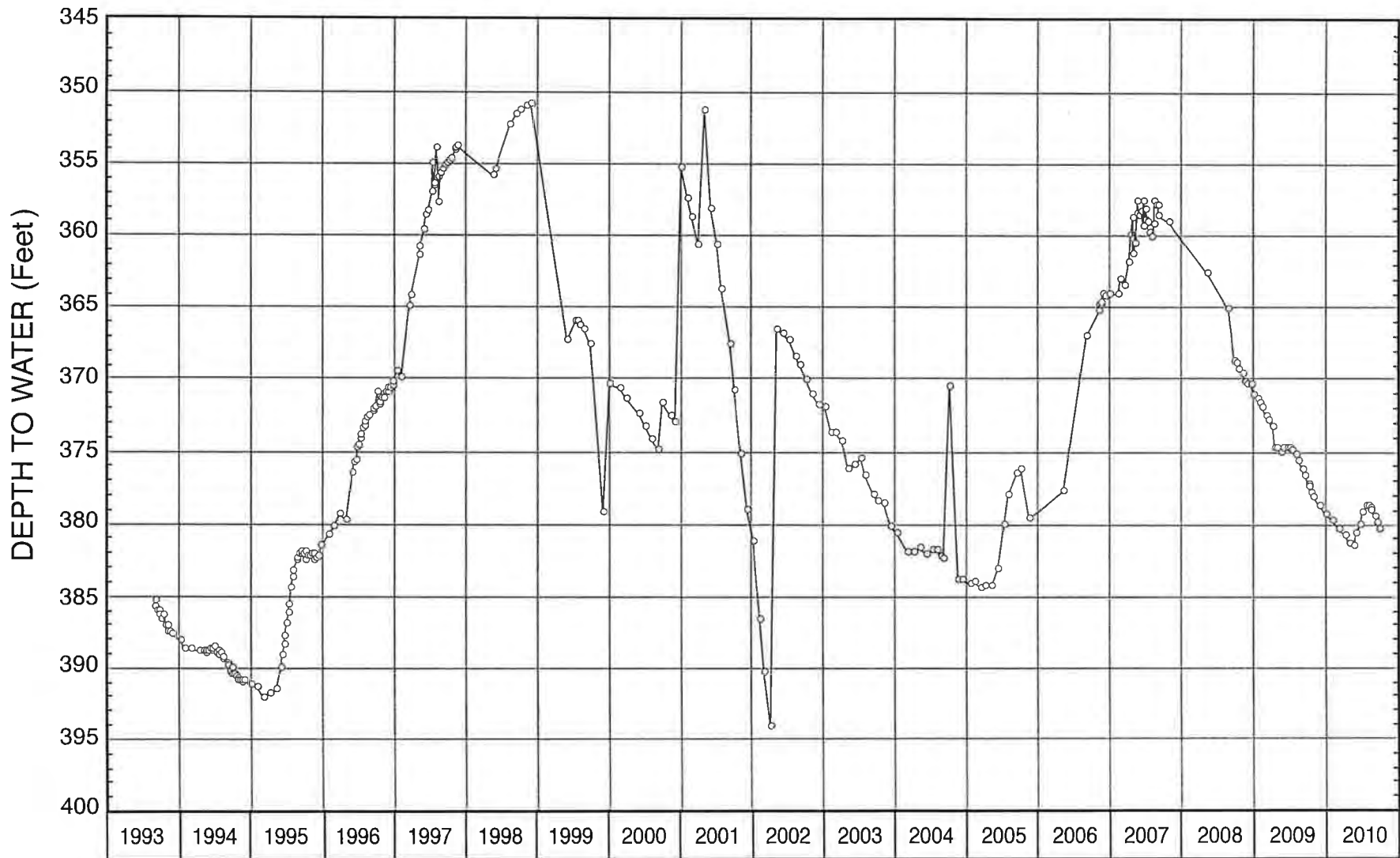
FIGURE 11 - WATER-LEVEL HYDROGRAPH FOR WELL NO. 24
