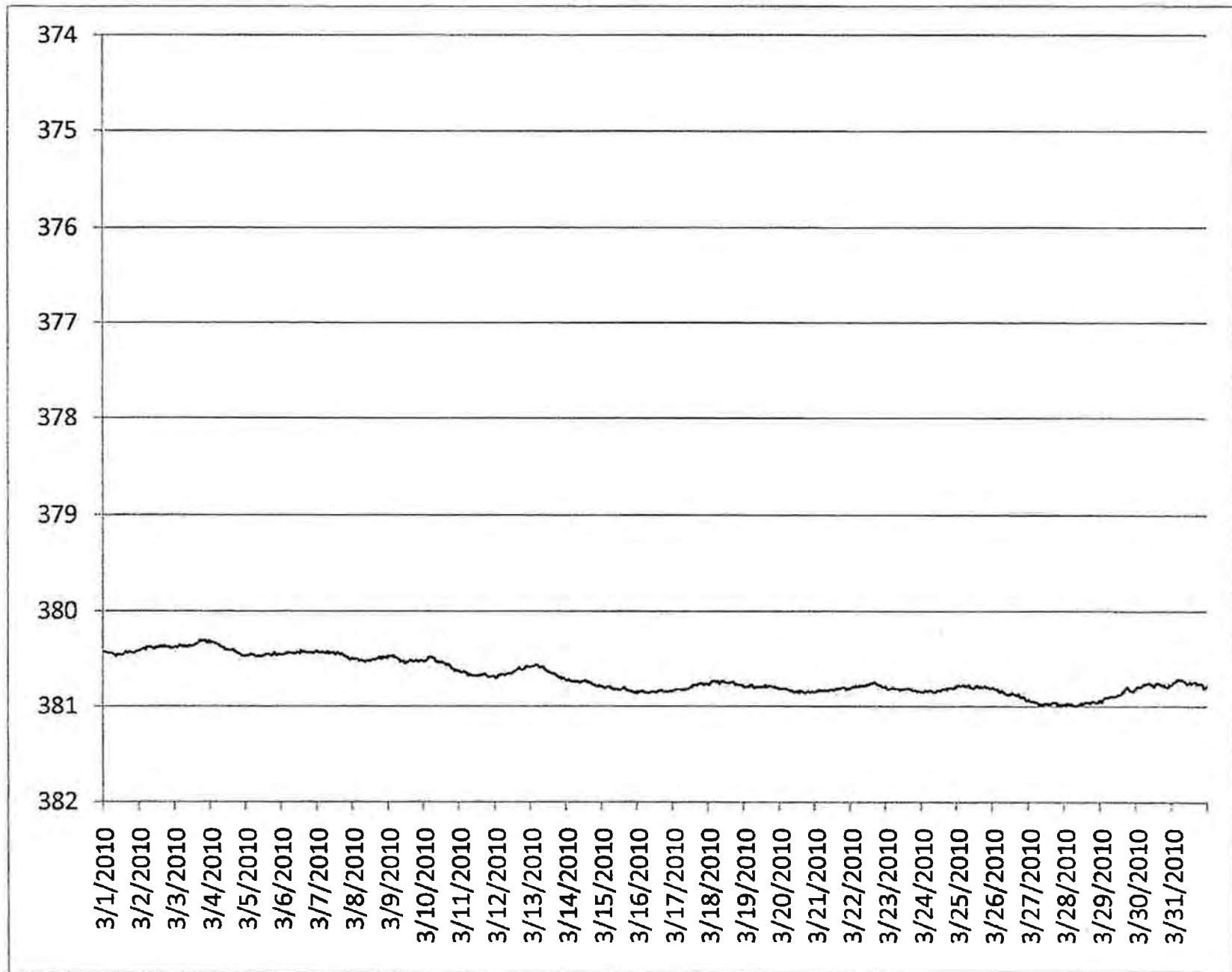
WATER LEVEL HYDROGRAPH FOR MW-24M
