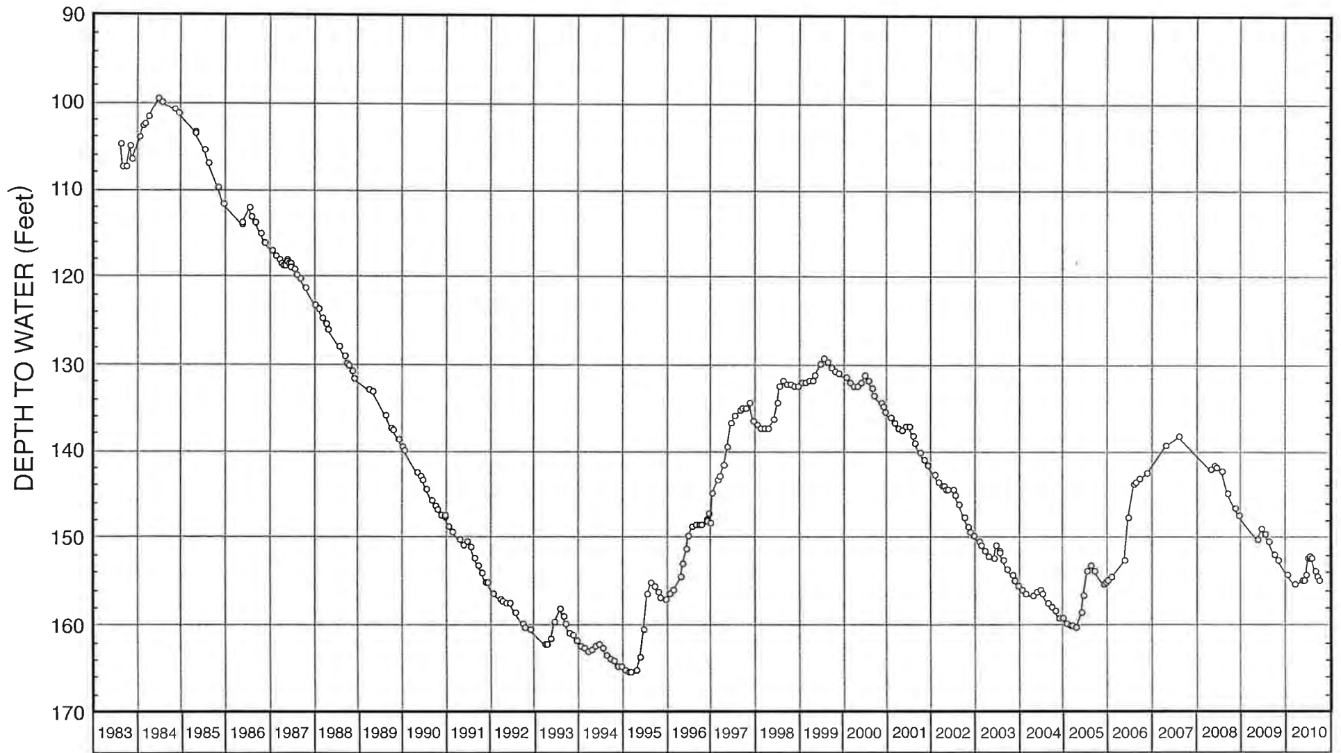
FIGURE 13 - WATER-LEVEL HYDROGRAPH FOR SC-2
