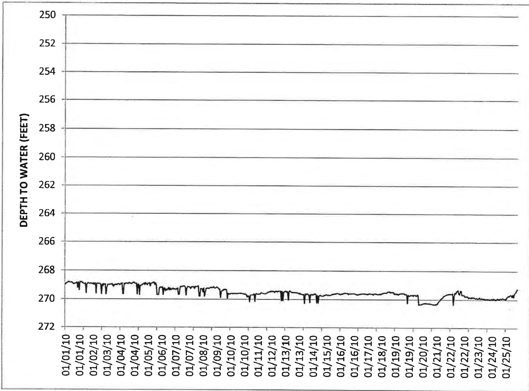
WATER LEVEL HYDROGRAPH FOR MW-26M
