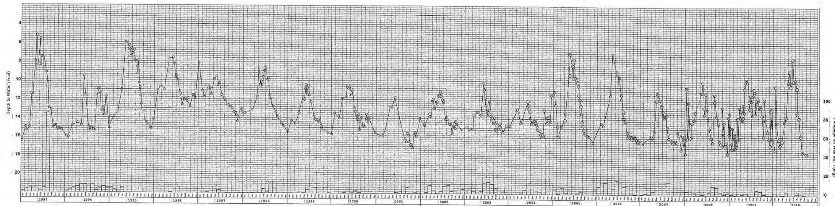
FIGURE 16-WATER-LEVEL HYDROGRAPH FOR WELL NO. 23 AND PUMPAGE FOR WELL NO. 1
