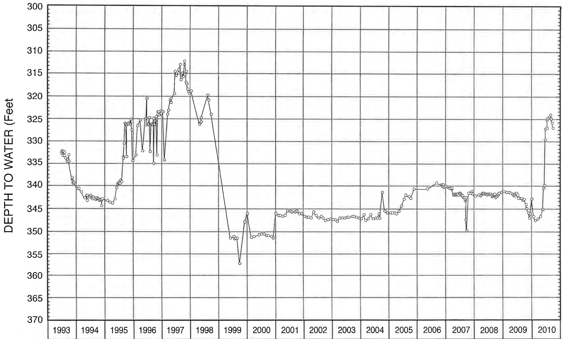
FIGURE 9 - WATER-LEVEL HYDROGRAPH FOR WELL NO. 19
