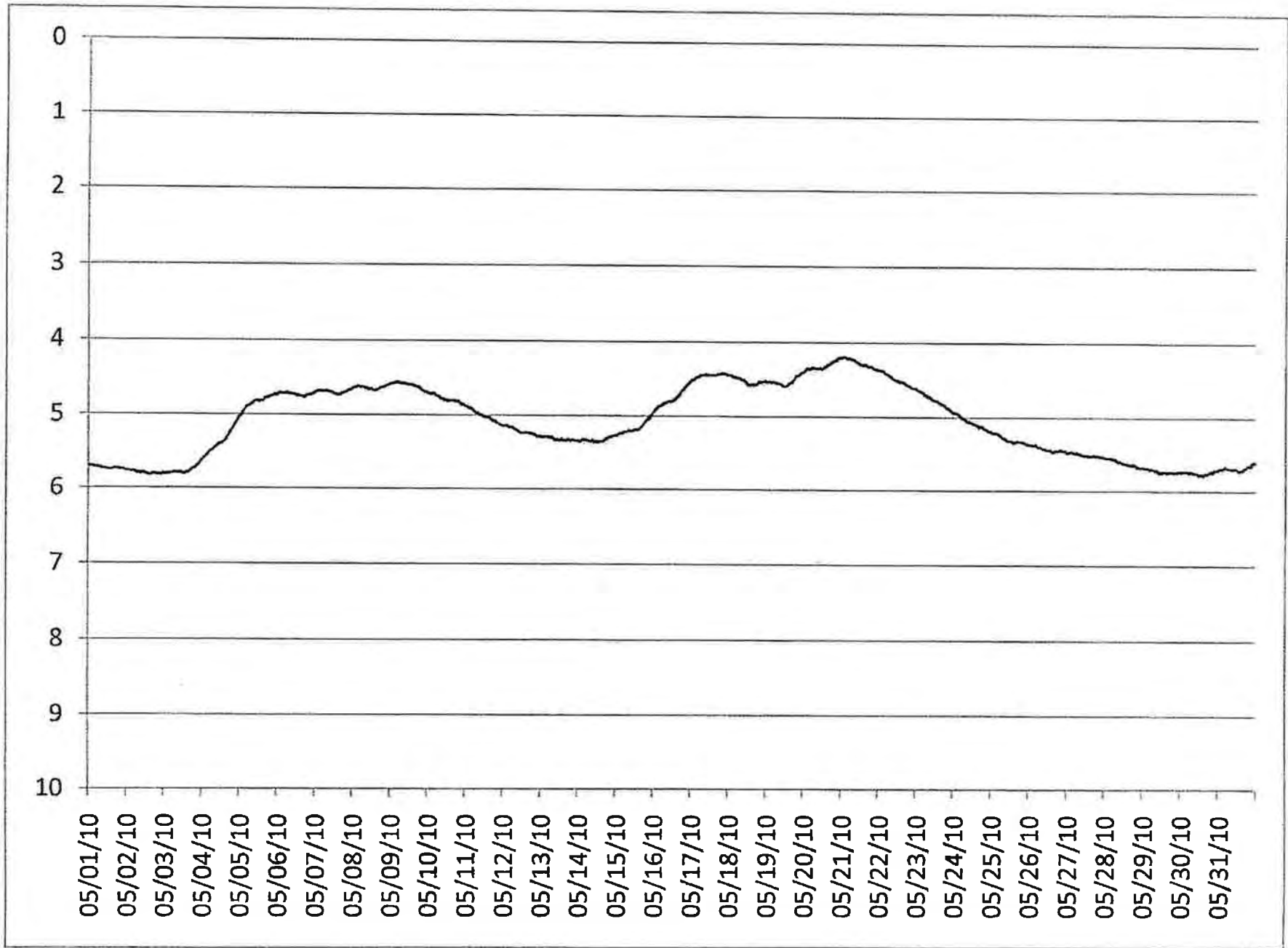
WATER LEVEL HYDROGRAPH FOR MW-5M
