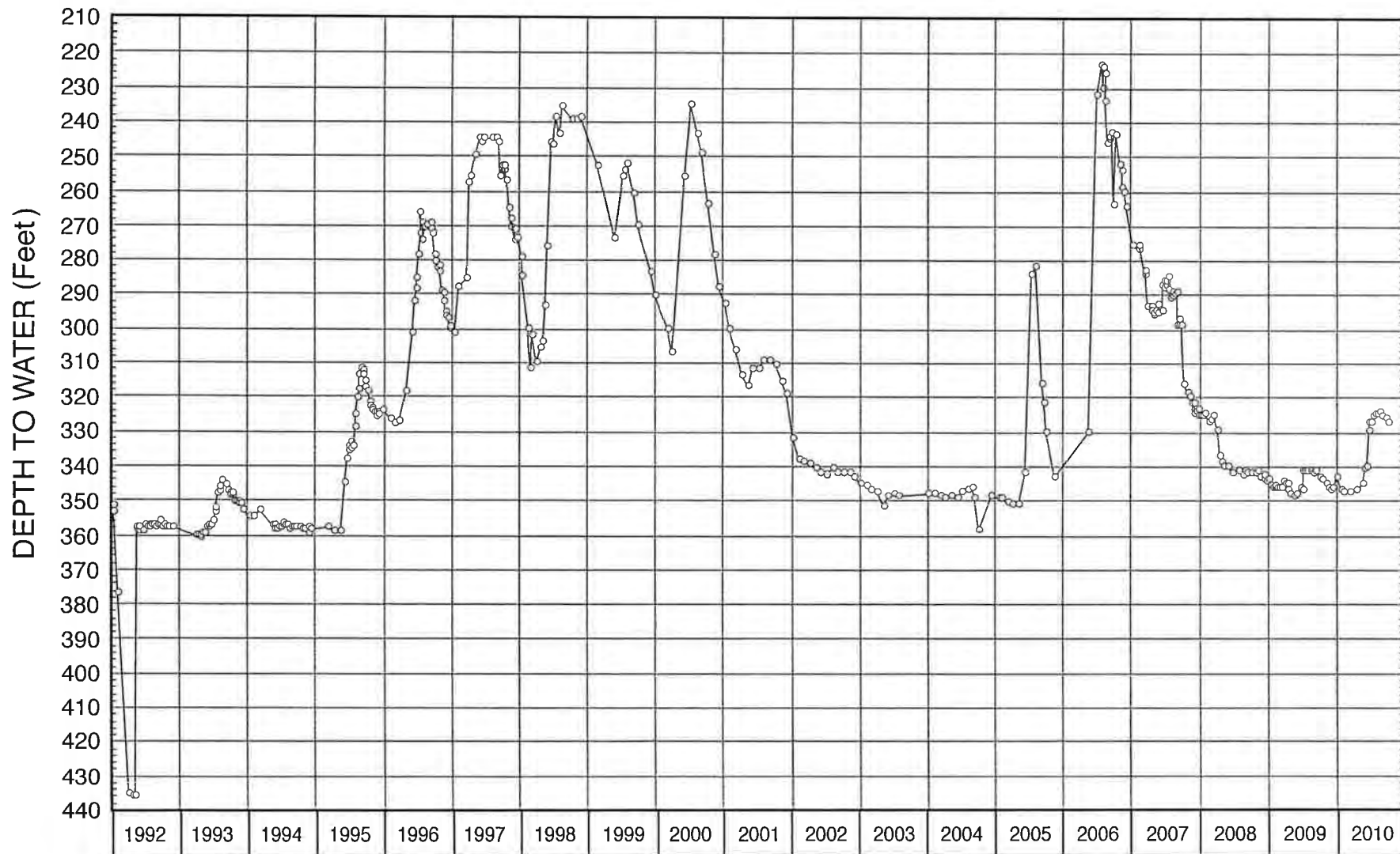
FIGURE 8 - WATER-LEVEL HYDROGRAPH FOR WELL NO. 14M
