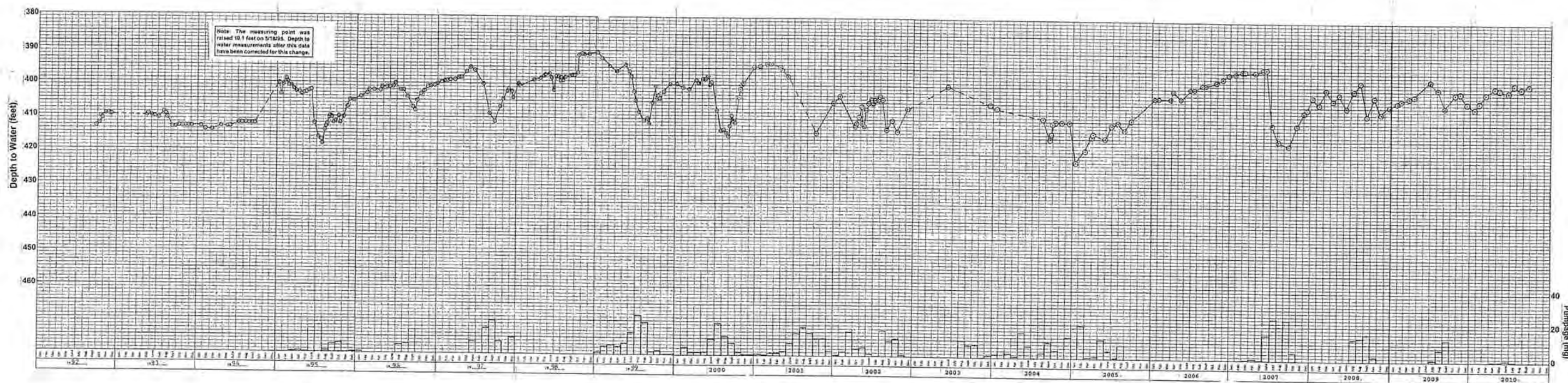
FIGURE 7-WATER-LEVEL AND PUMPAGE HYDROGRAPH FOR WELL NO. 20
