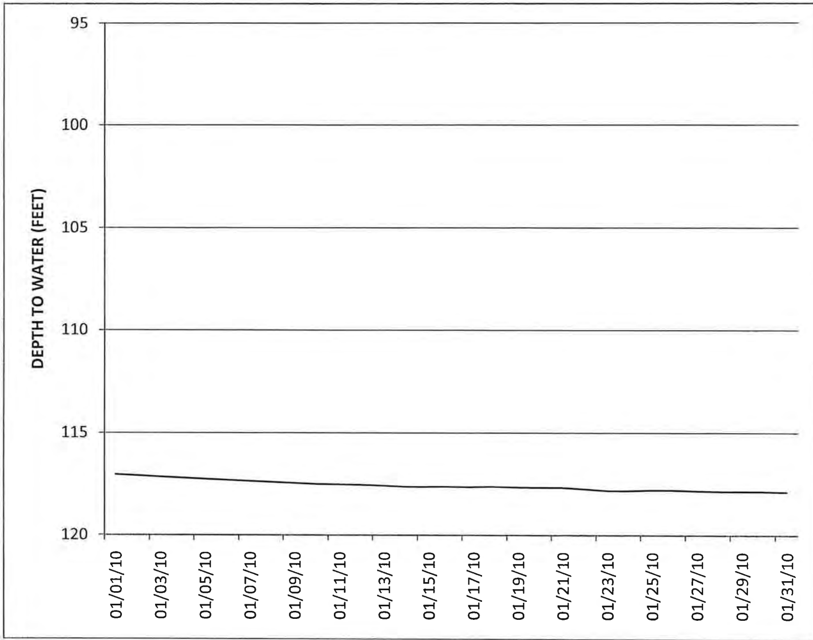
WATER LEVEL HYDROGRAPH FOR SC-1
