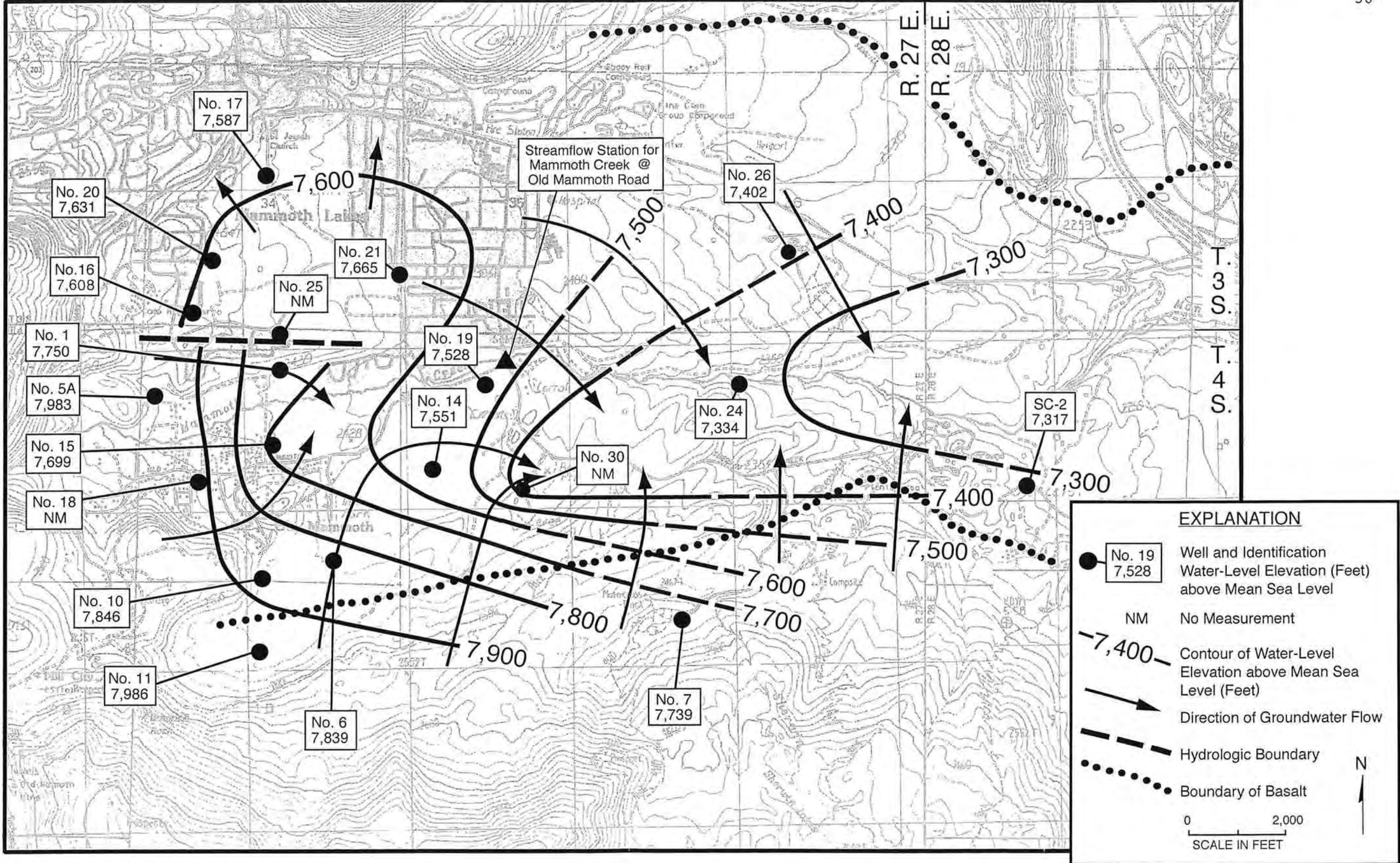
FIGURE 18 - WATER-LEVEL ELEVATIONS IN SEPTEMBER 2010
