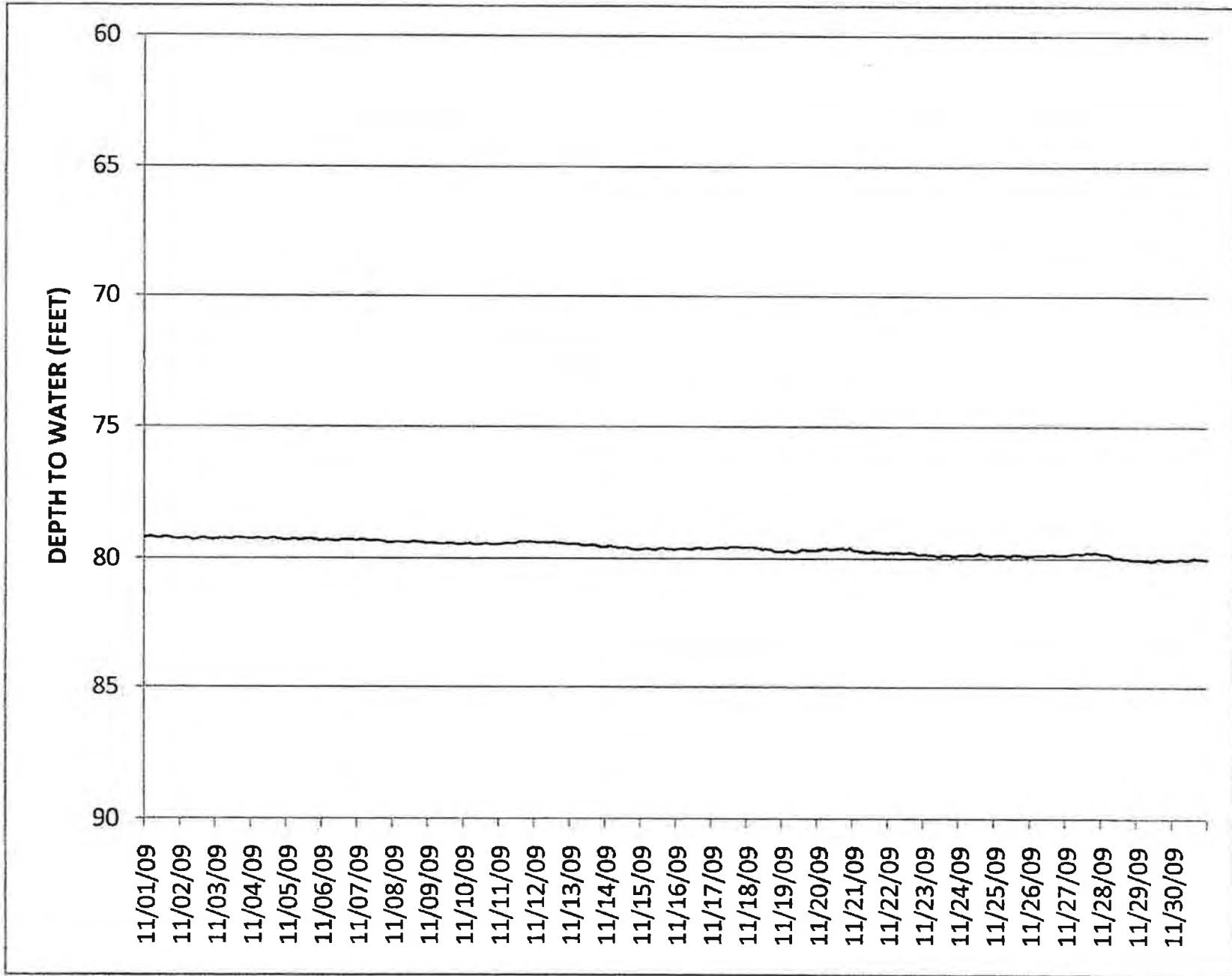
WATER LEVEL HYDROGRAPH FOR MW-28M
