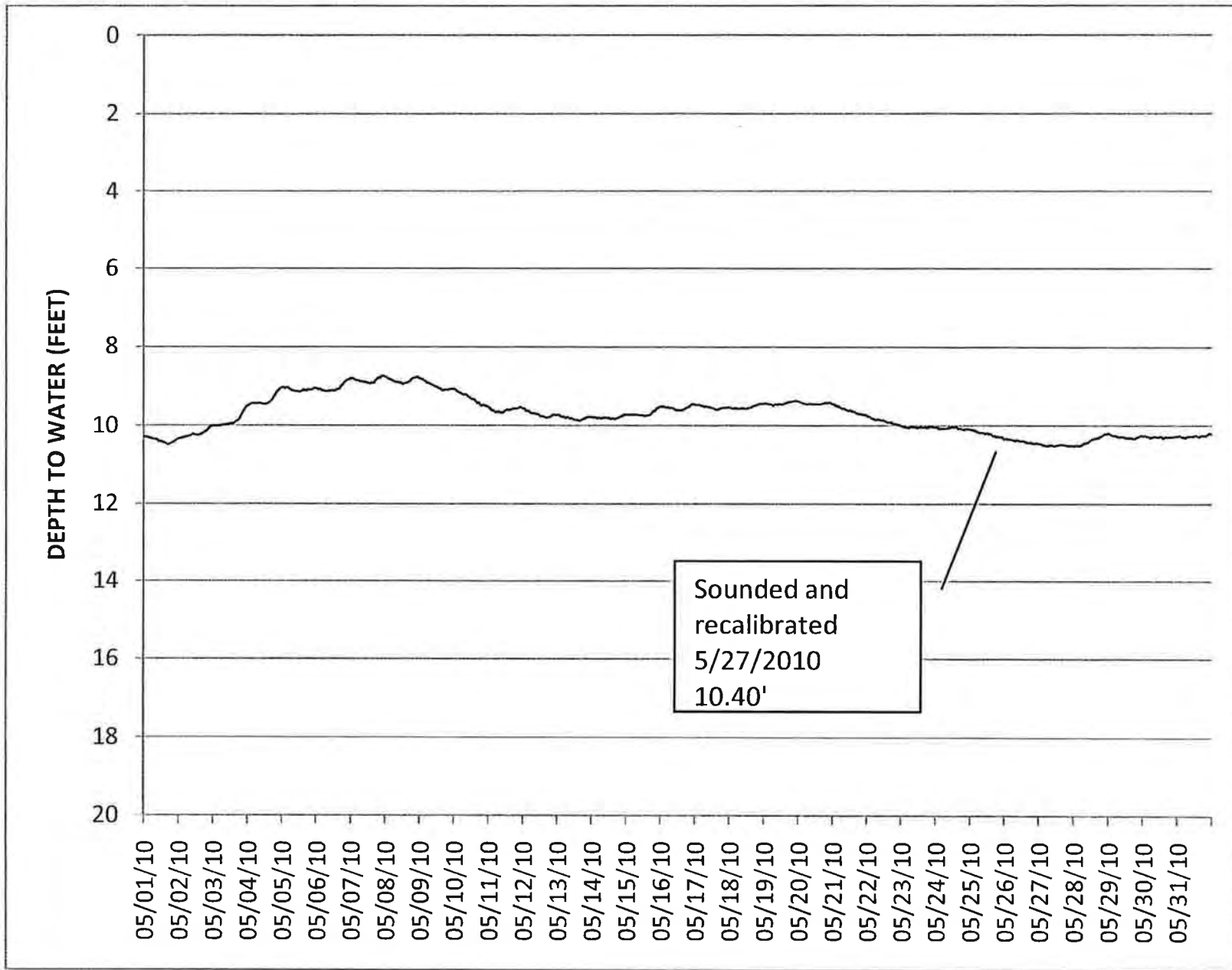
WATER LEVEL HYDROGRAPH FOR MW-23M
