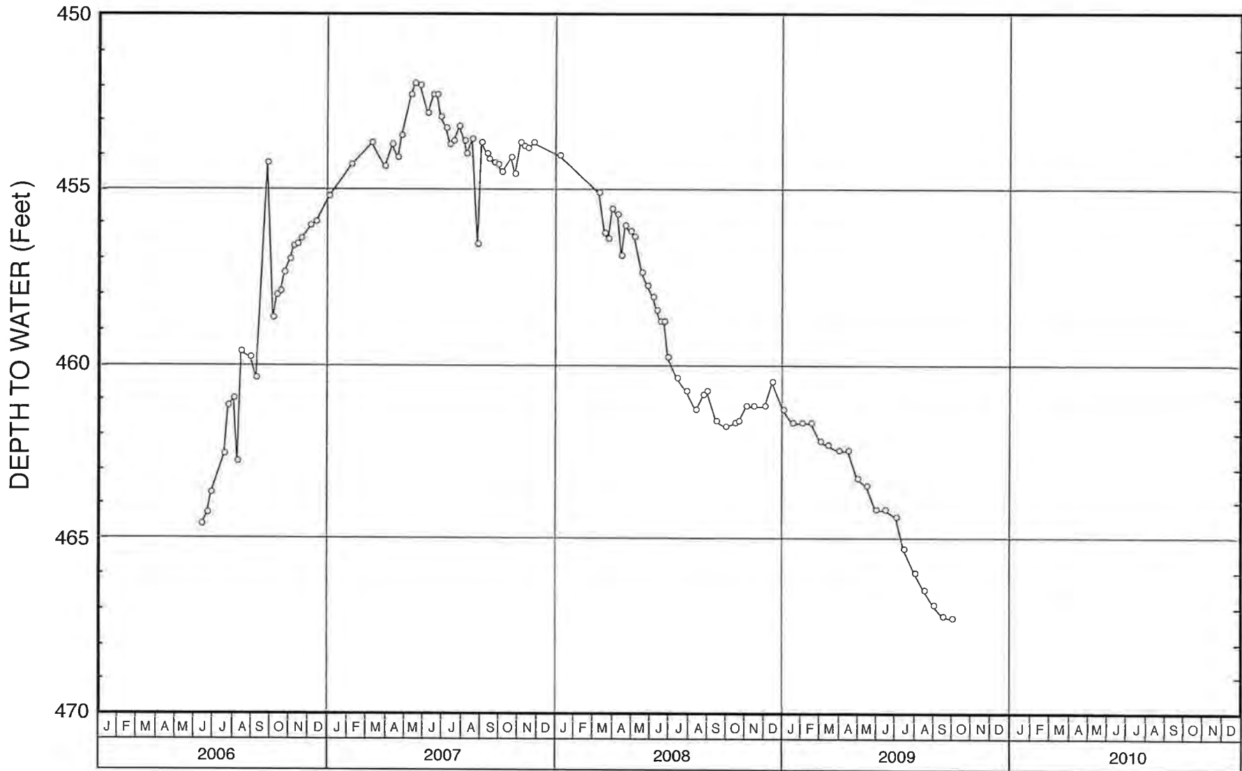
WATER-LEVEL HYDROGRAPH FOR WELL NO. 30
