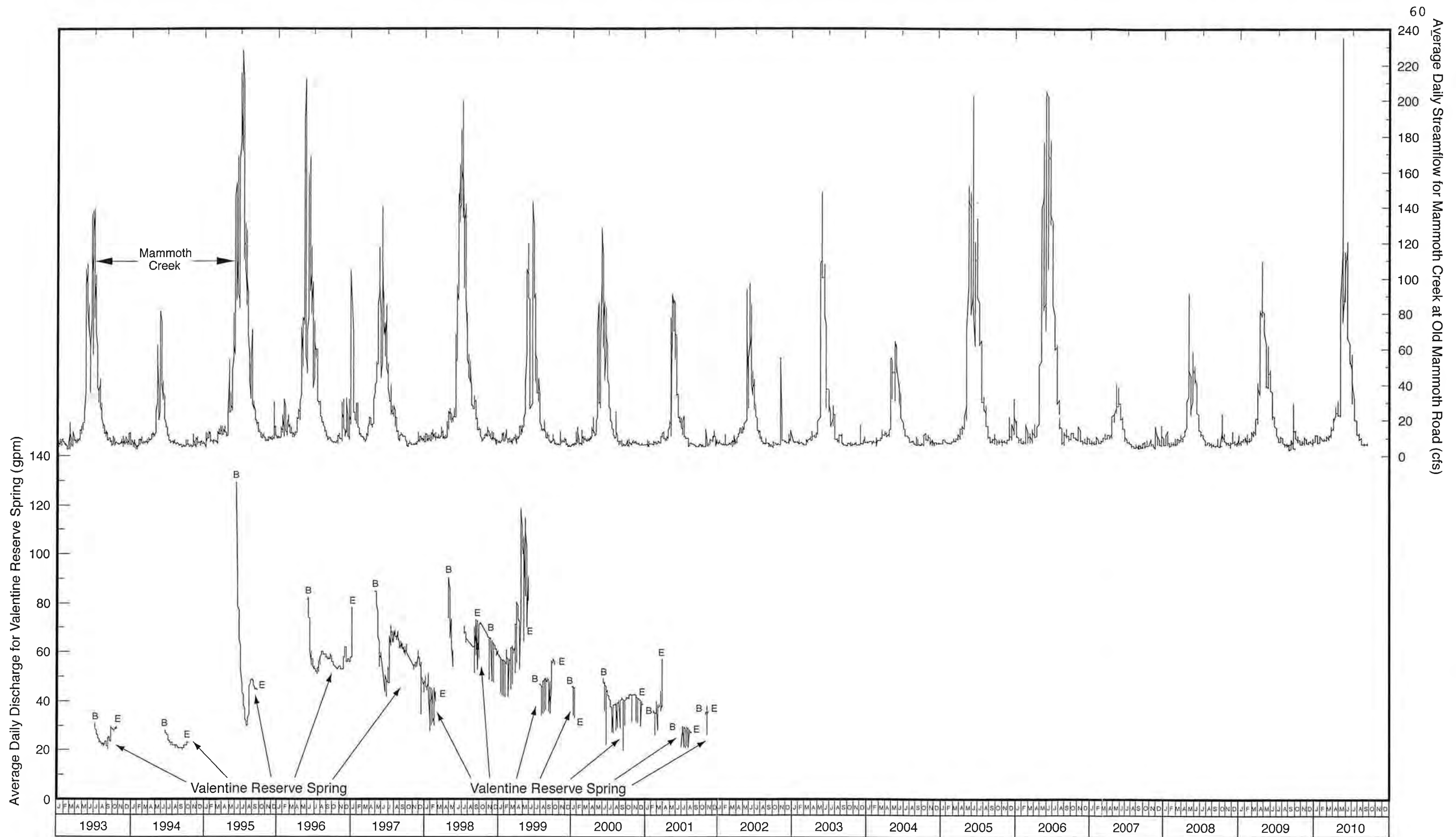
FIGURE 19 - FLOW FOR VALENTINE SPRING (1993-2001) AND MAMMOTH CREEK STREAMFLOW (1993-2010)
