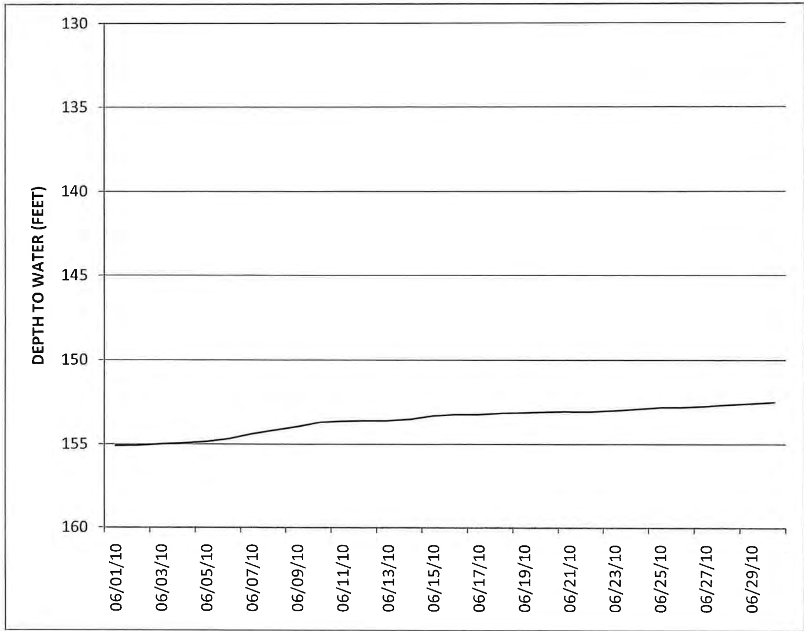
WATER LEVEL HYDROGRAPH FOR SC-2
