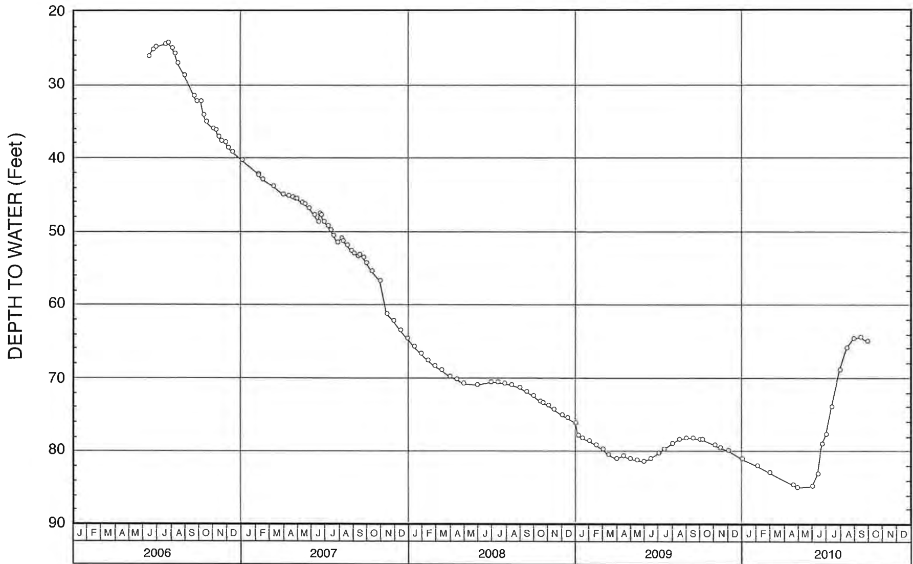
WATER-LEVEL HYDROGRAPH FOR WELL NO. 28
