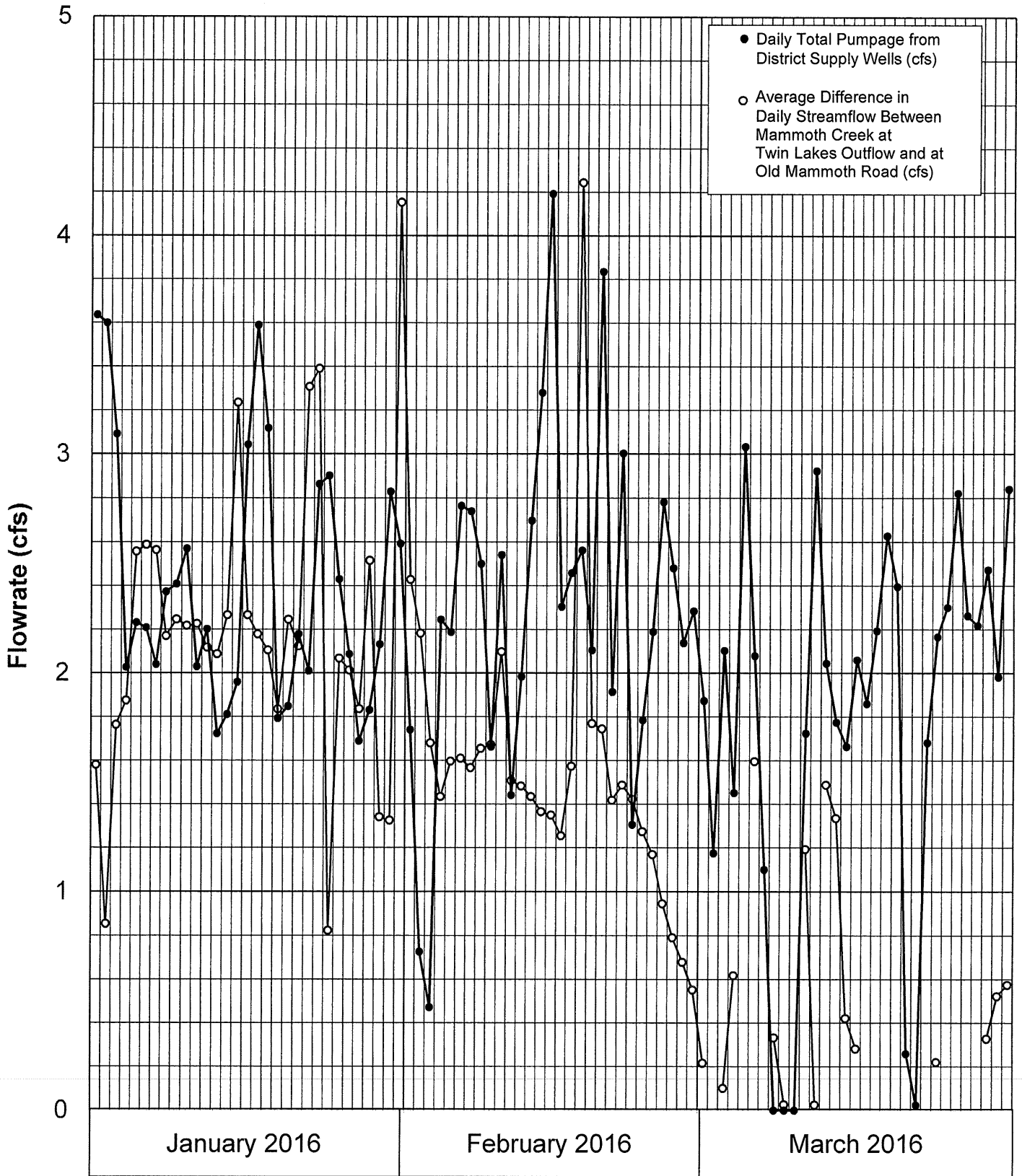
FIGURE 21-RELATIONSHIP BETWEEN DIFFERENCE IN MAMMOTH CREEK STREAMFLOW AT TWIN LAKES OUTFLOW AND OLD MAMMOTH ROAD AND DISTRICT SUPPLY WELL PUMPAGE (JANUARY-MARCH, 2016)
