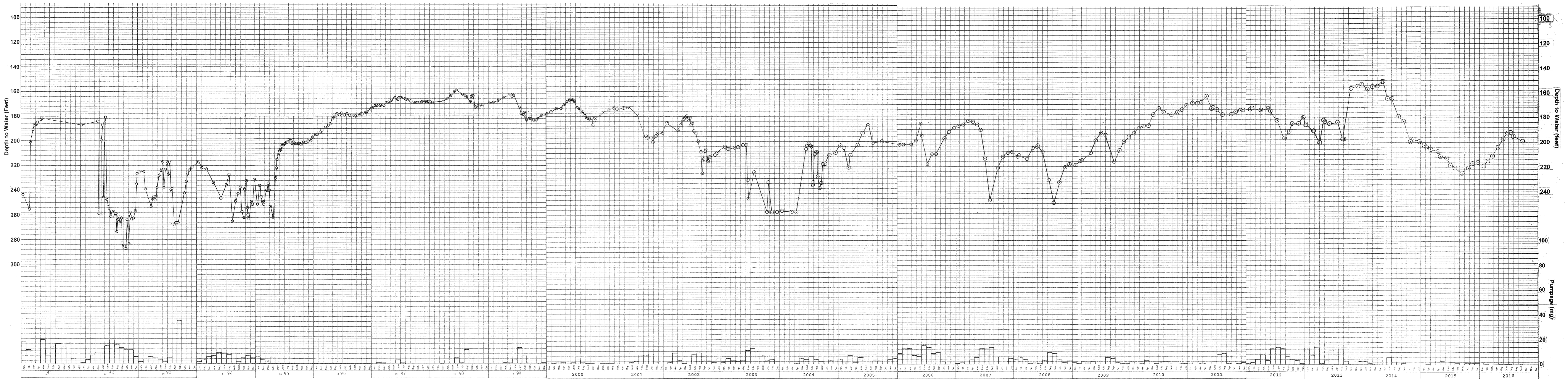
WATER-LEVEL AND PUMPAGE HYDROGRAPH FOR WELL NO. 1
