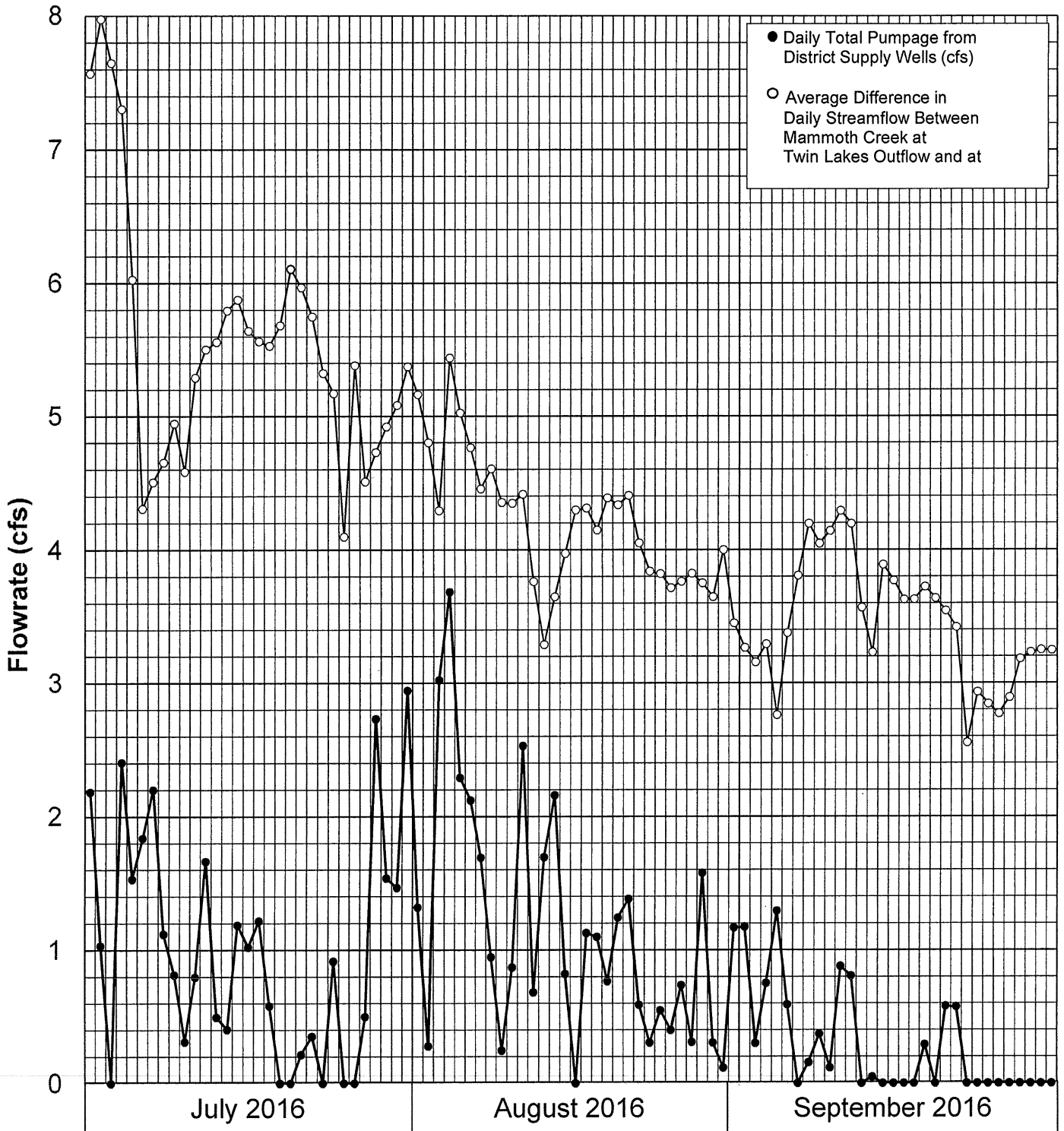
FIGURE 23-RELATIONSHIP BETWEEN DIFFERENCE IN MAMMOTH CREEK STREAMFLOW AT TWIN LAKES OUTFLOW AND OLD MAMMOTH ROAD AND DISTRICT SUPPLY WELL PUMPAGE (JULY-SEPTEMBER, 2016)
