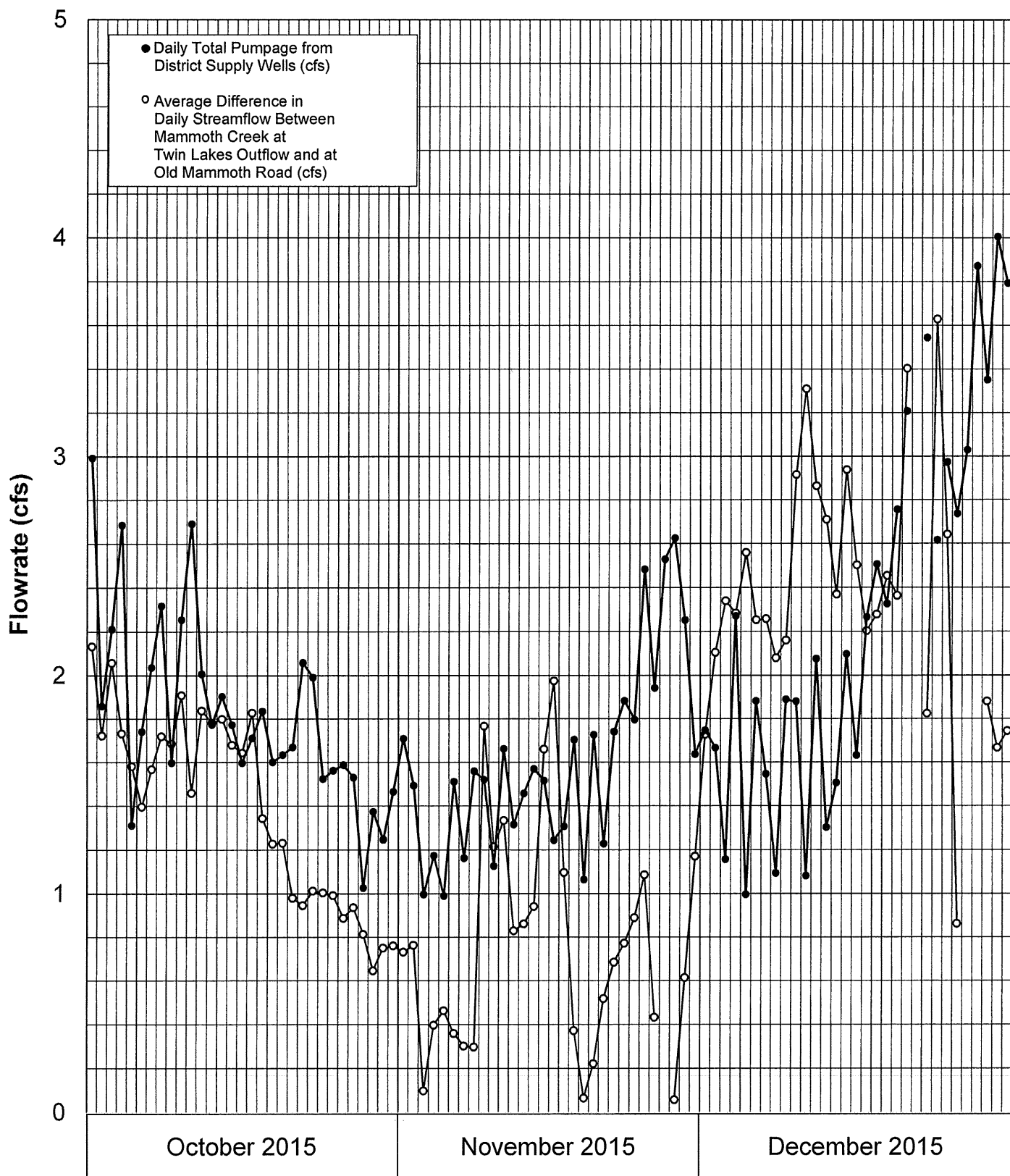
FIGURE 20-RELATIONSHIP BETWEEN DIFFERENCE IN MAMMOTH CREEK STREAMFLOW AT TWIN LAKES OUTFLOW AND OLD MAMMOTH ROAD AND DISTRICT SUPPLY WELL PUMPAGE (OCTOBER-DECEMBER, 2015)
