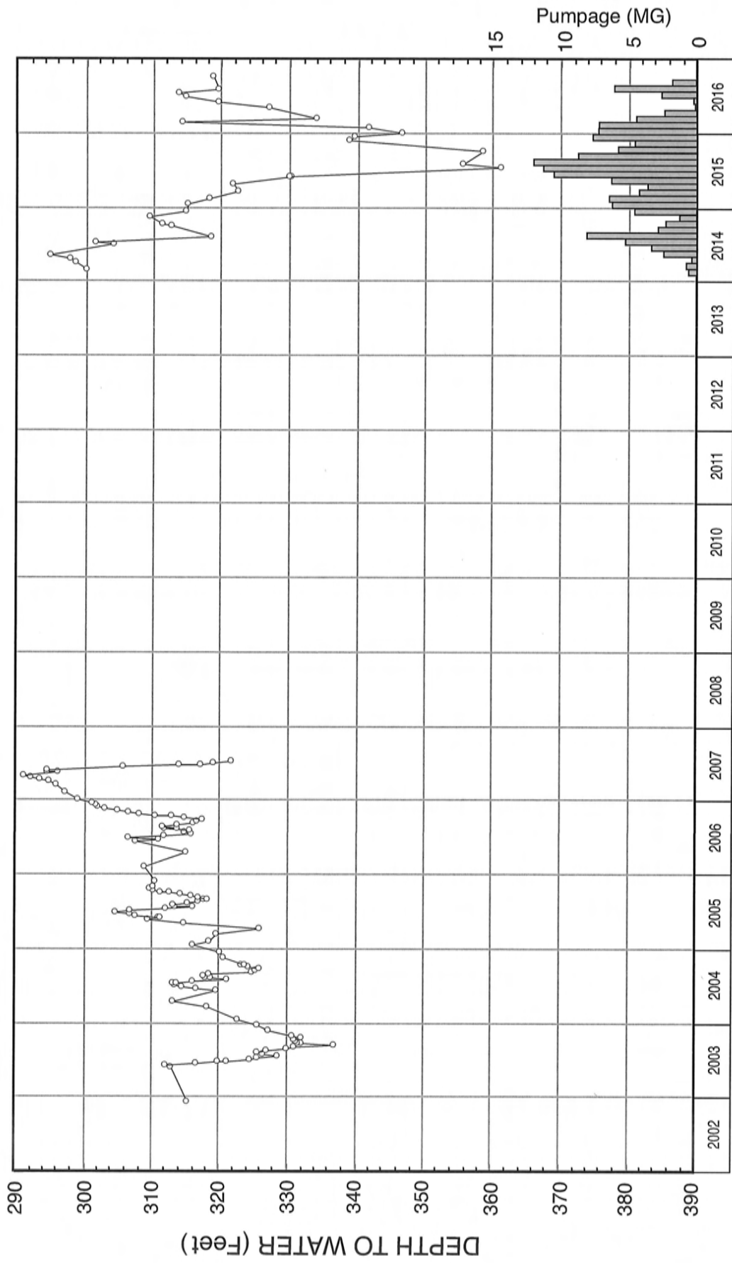
FIGURE 8 - WATER-LEVEL HYDROGRAPH FOR WELL NO. 25
