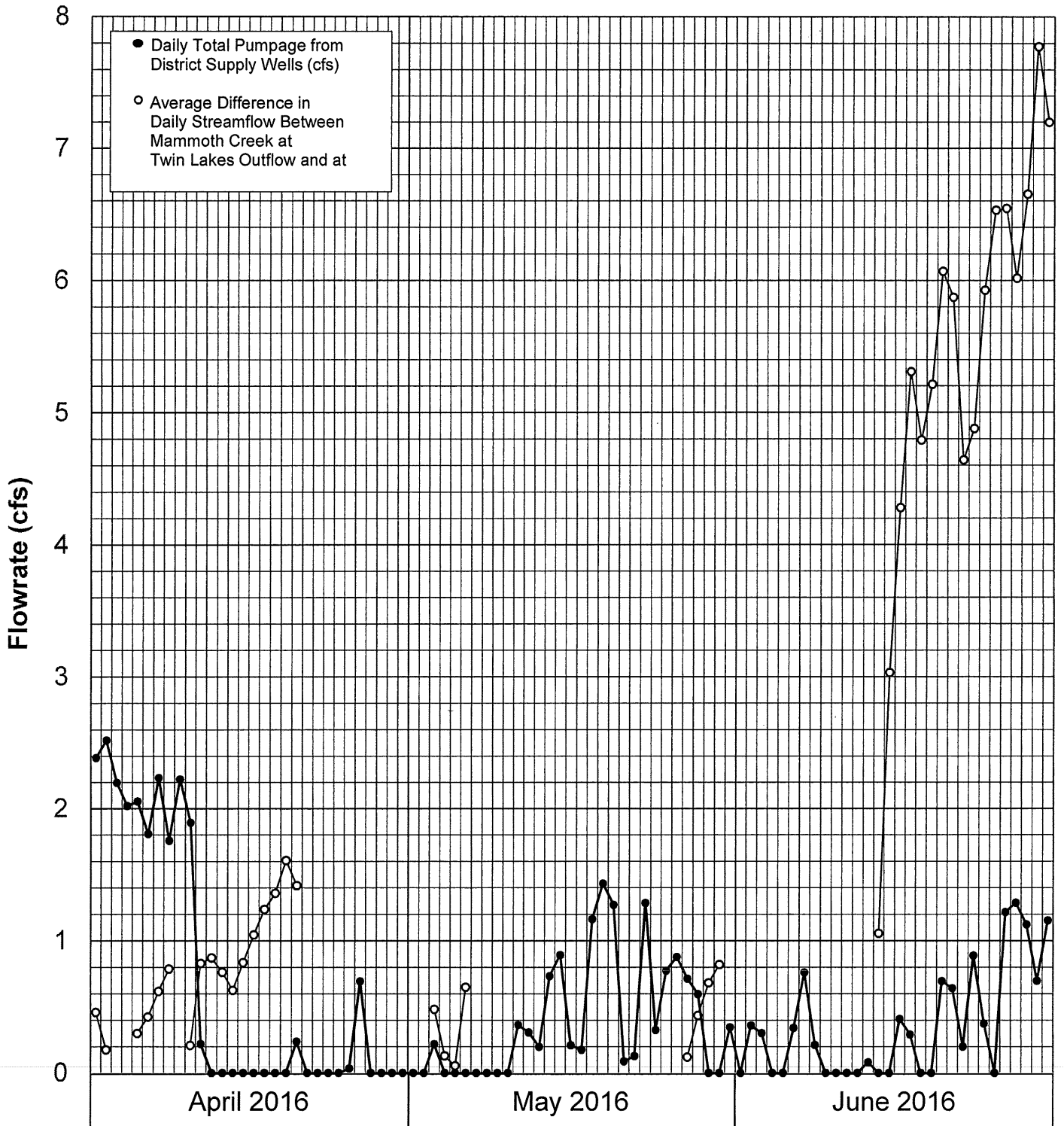
FIGURE 22-RELATIONSHIP BETWEEN DIFFERENCE IN MAMMOTH CREEK STREAMFLOW AT TWIN LAKES OUTFLOW AND OLD MAMMOTH ROAD AND DISTRICT SUPPLY WELL PUMPAGE (APRIL-JUNE, 2016)
