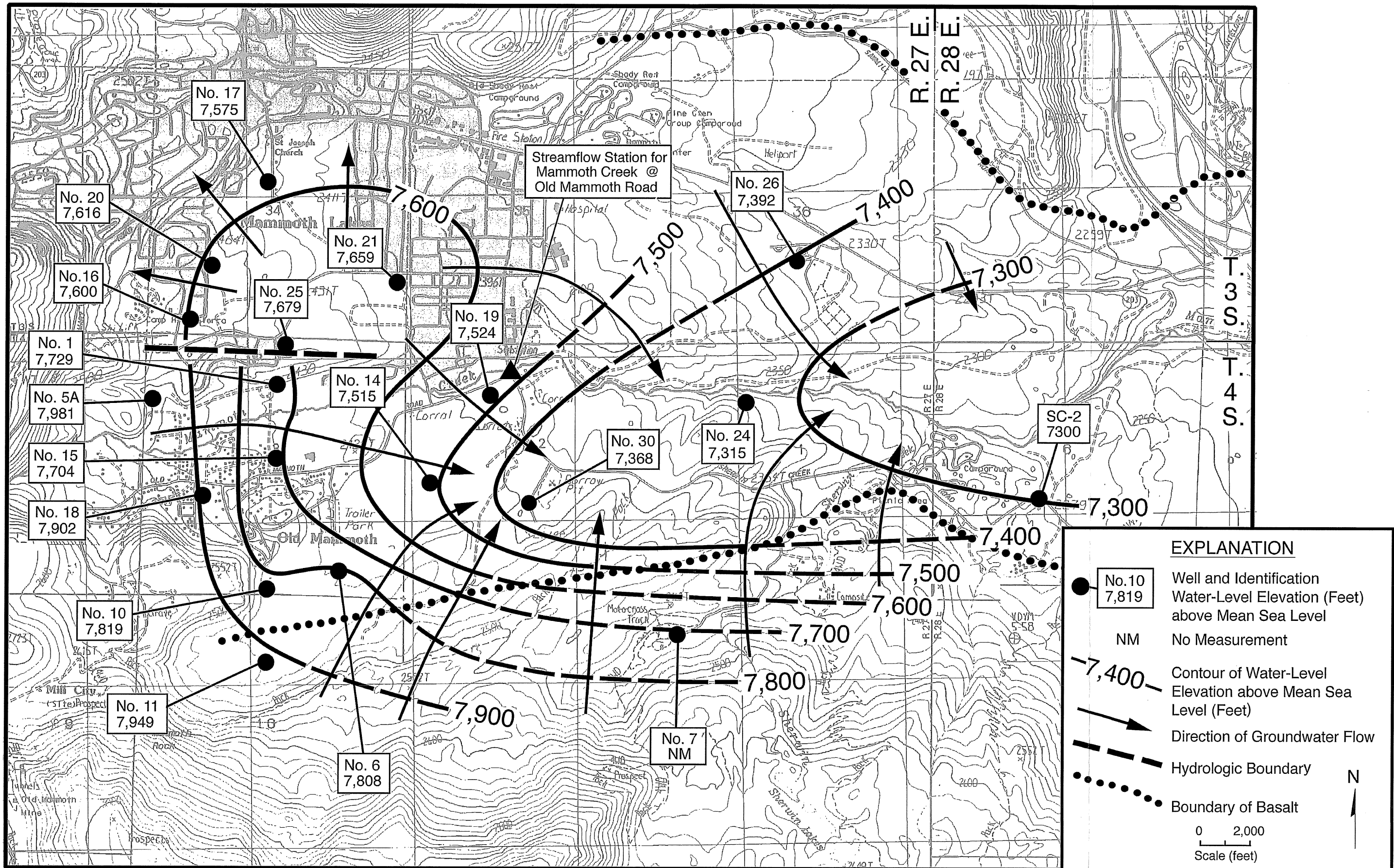
FIGURE 19 - WATER-LEVEL ELEVATIONS IN LATE SEPTEMBER 2016
