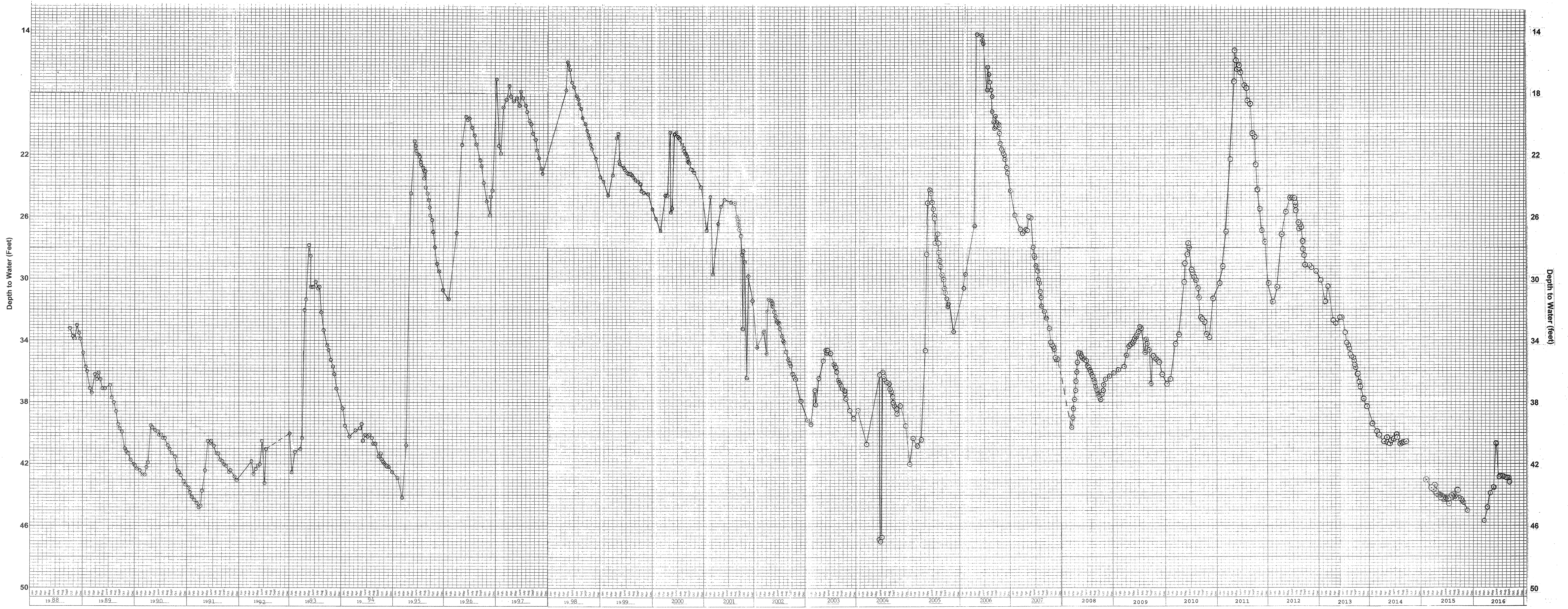
WATER-LEVEL HYDROGRAPH FOR WELL NO. 4M
