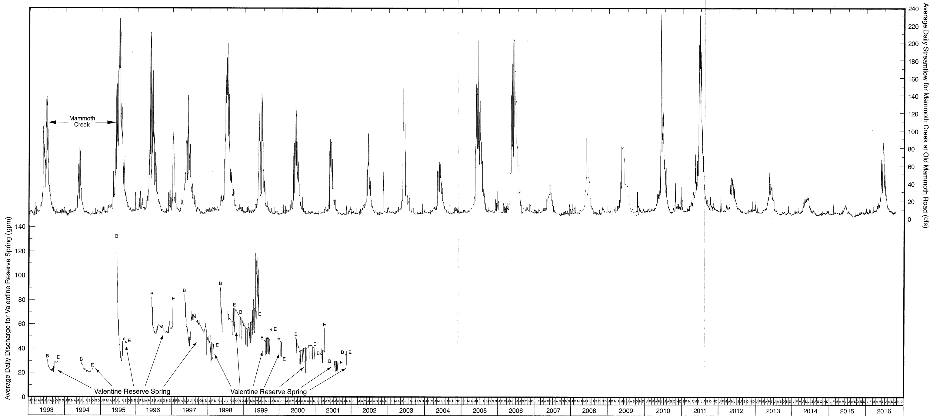
FIGURE 24 - FLOW FOR VALENTINE SPRING (1993-2001) AND MAMMOTH CREEK STREAMFLOW (1993-2016)
