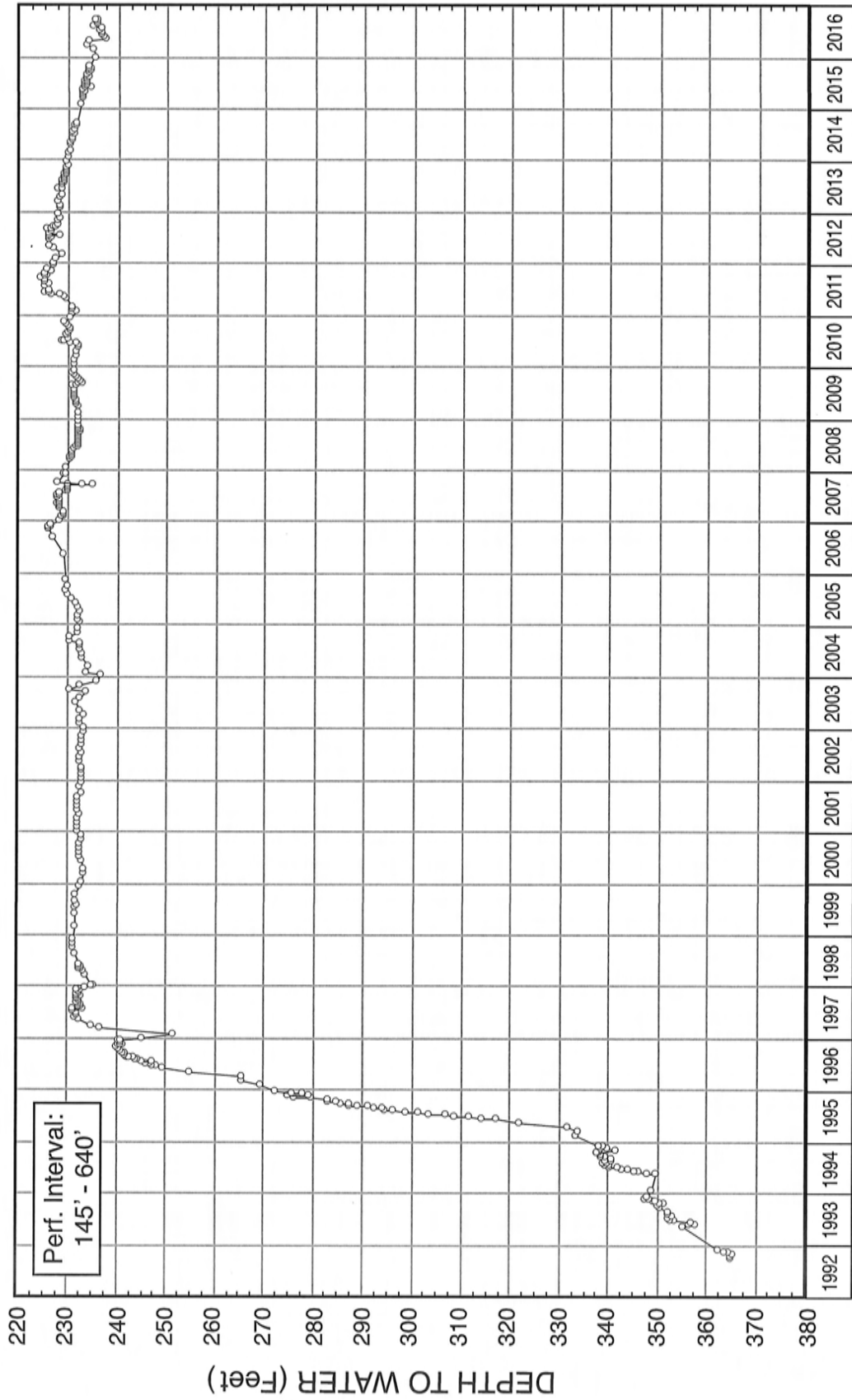
FIGURE 11 - WATER-LEVEL HYDROGRAPH FOR WELL NO. 21
